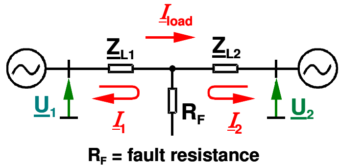
Fig. 1: Simple model for the effect of fault resistance at double-ended infeed (load flow from left to right)
